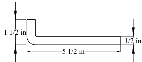
HANGER DETAIL (1/2 in x 1/2 in SQUARE)
